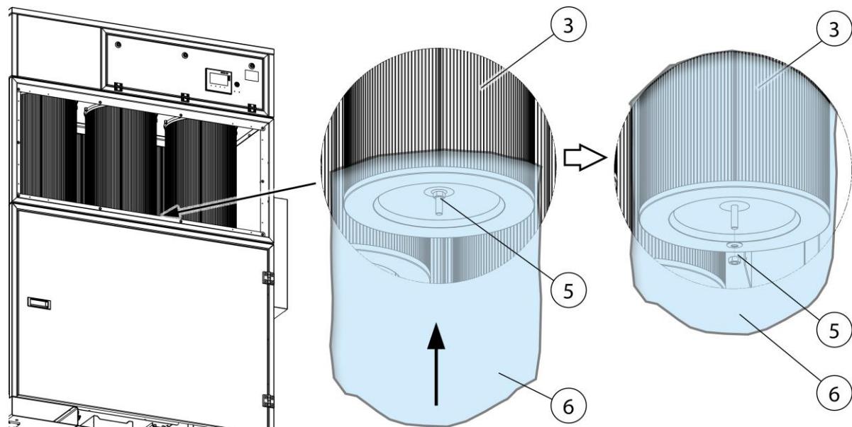
Fig. 44: Changing filters -
