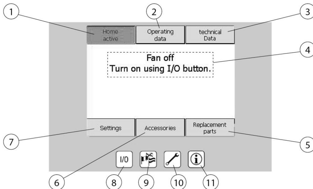
Fig. 20: Operating elements
