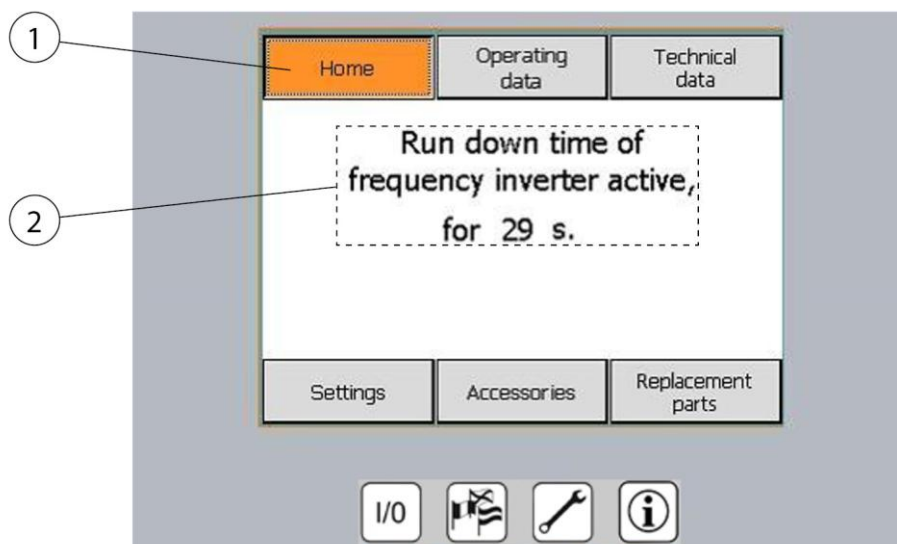
Fig. 8: Run-down time
