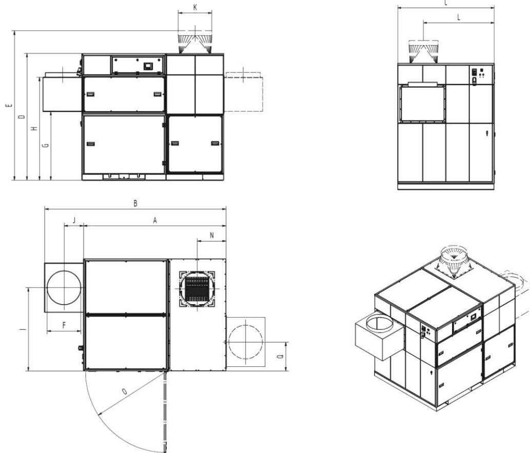
Fig. 64: Dimension sheet 3250110, 3250112, 3265111, 3265112
